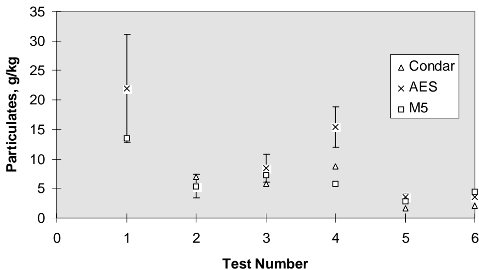
Figure 11. Comparison of masonry fireplace PM emission factors as measured by three different test methods
