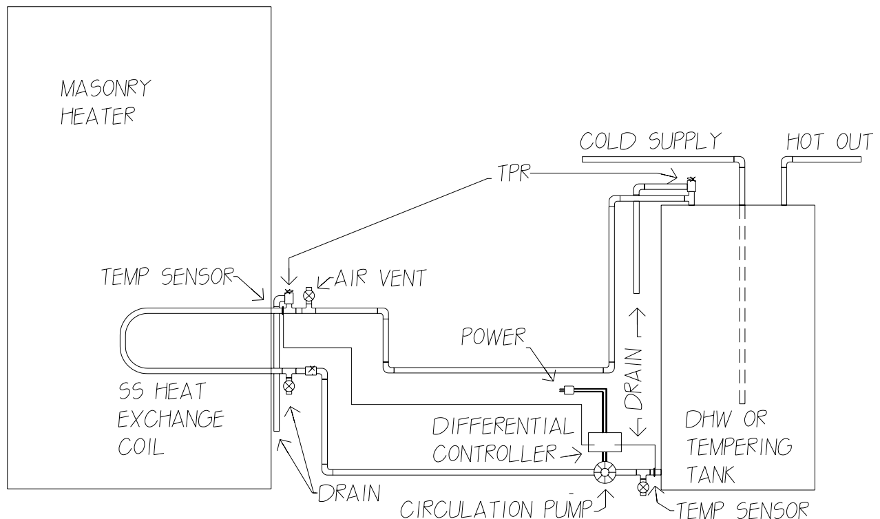
Figure 7. Hot water system—circulation pump method
