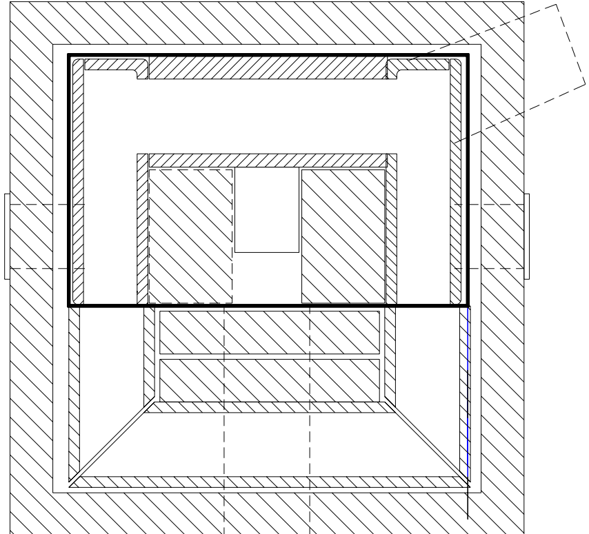
Figure 8. Heated bench layout for contraflow heater
