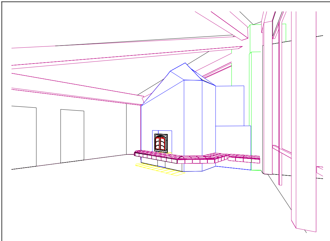
Figure 4. Masonry heating system at Kitchener-Waterloo YMCA Earth Residence. Design output is 15kW including 2000 litres of DHW/day. Fuel requirement at maximum output is 300 lb/day.
