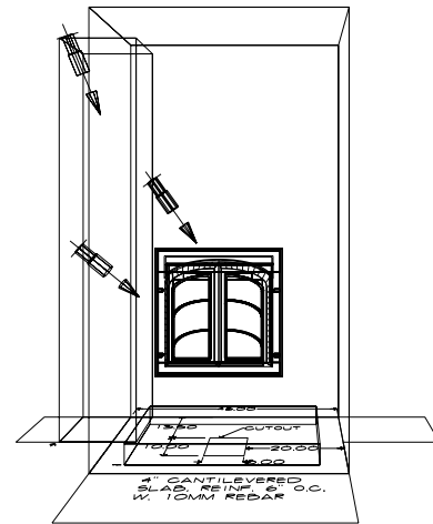
Figure 5. Masonry heating system layout for Crainford residence
